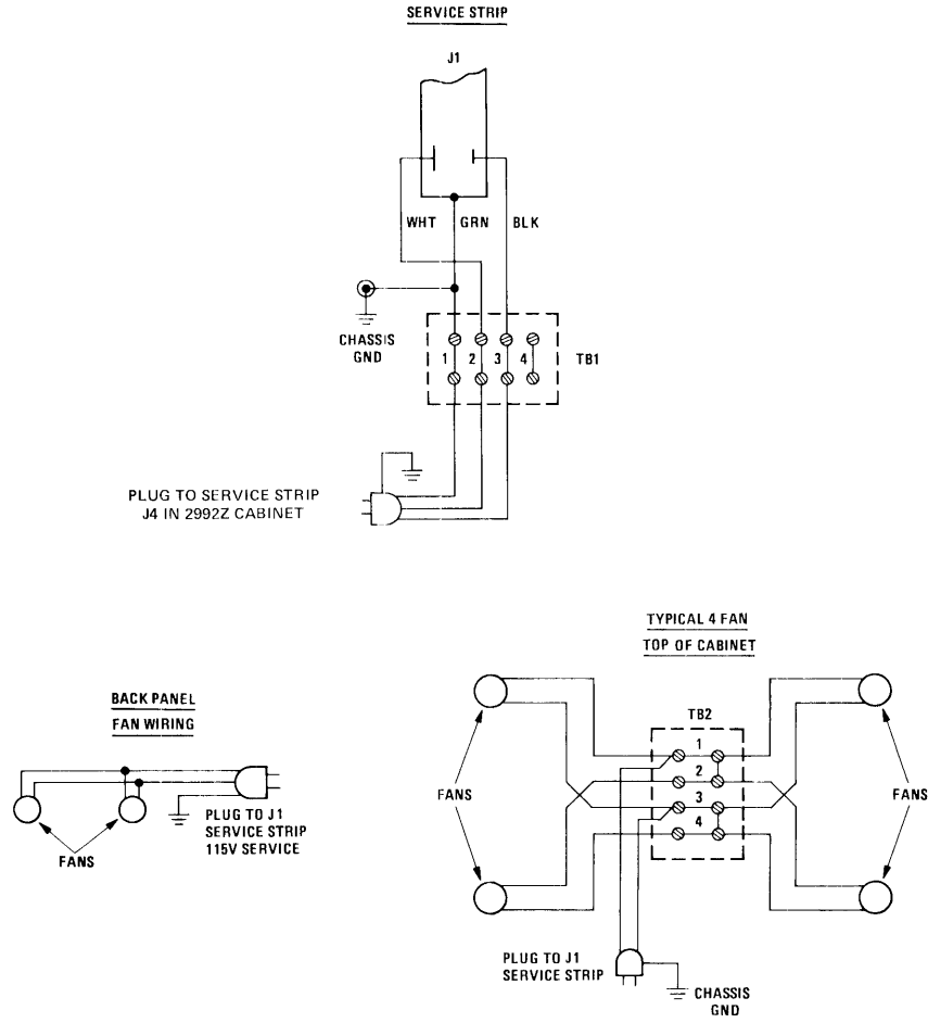
Figure 3-2. HP 2866A Extender Cabinet Wiring Diagram
