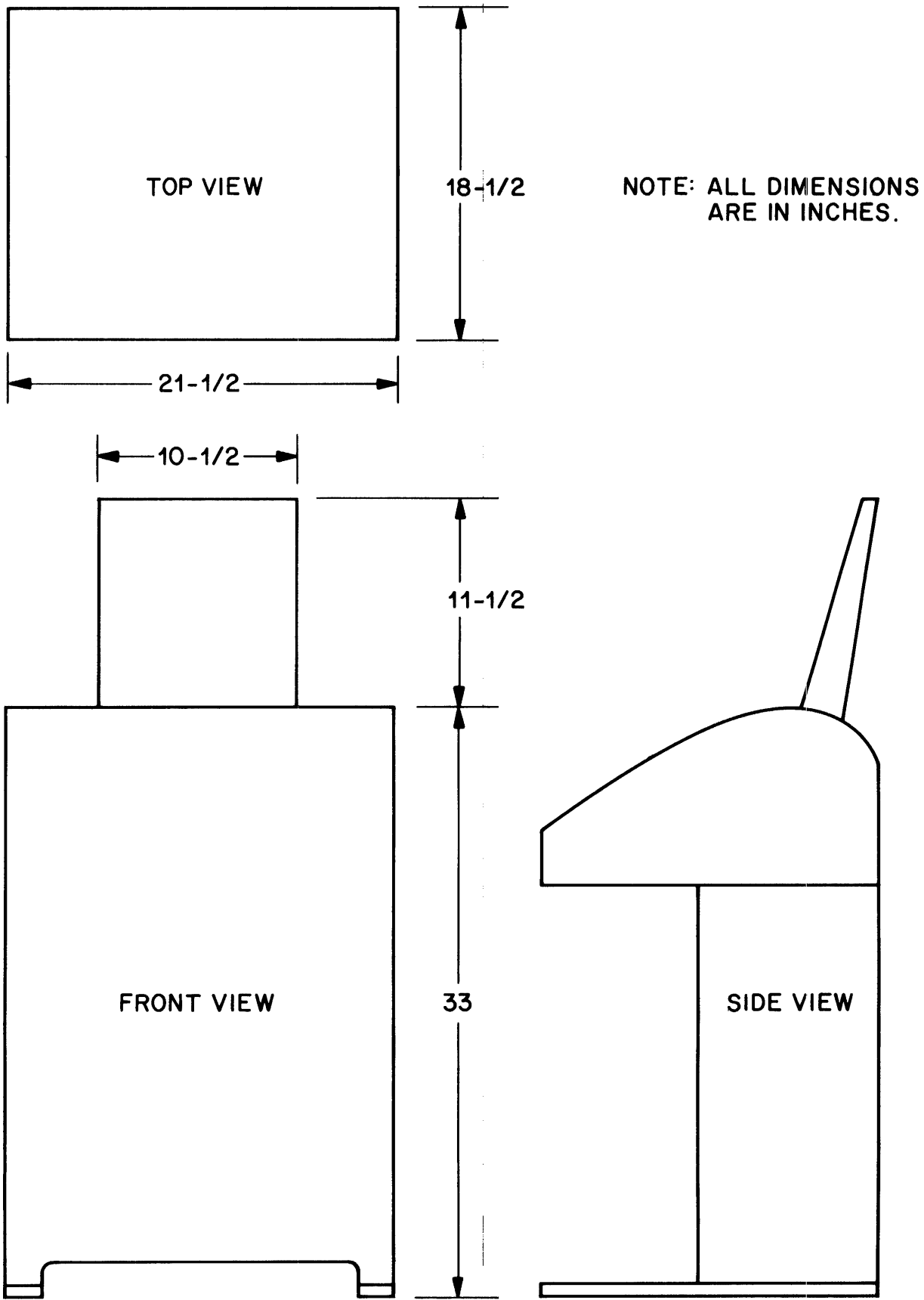
Figure 2-16. HP 2749A Teleprinter Outline Drawing
