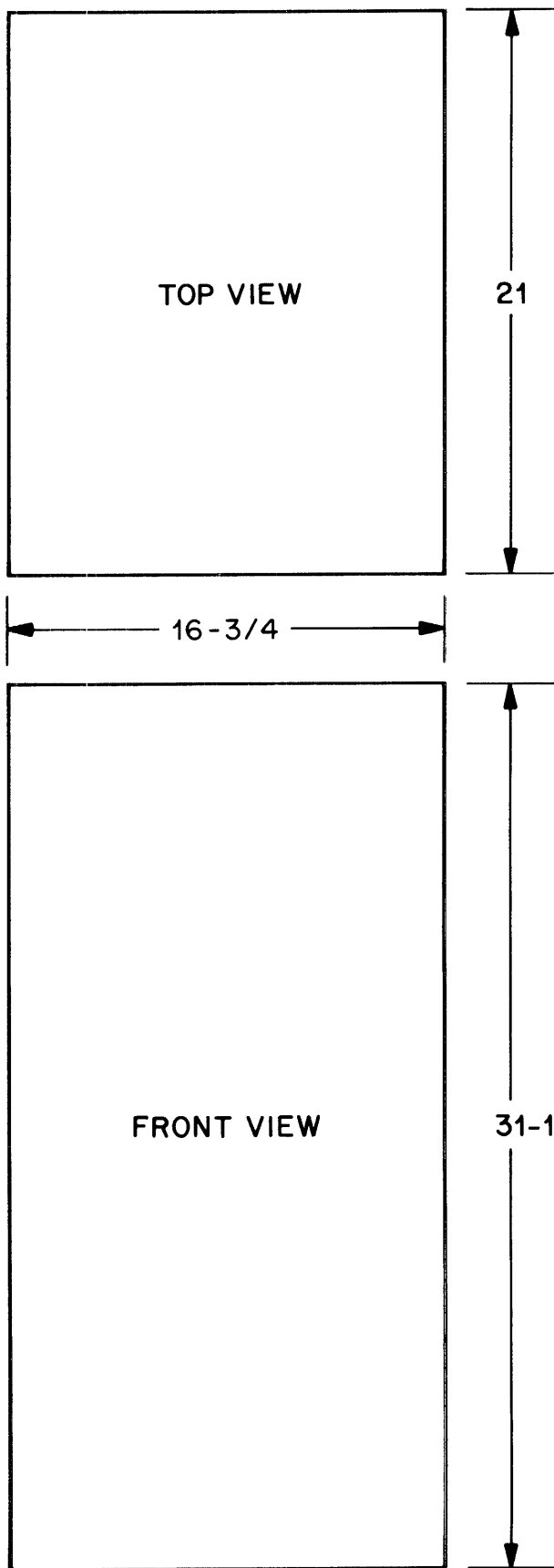
Figure 2-34. HP 2150B Extender Outline Drawing
