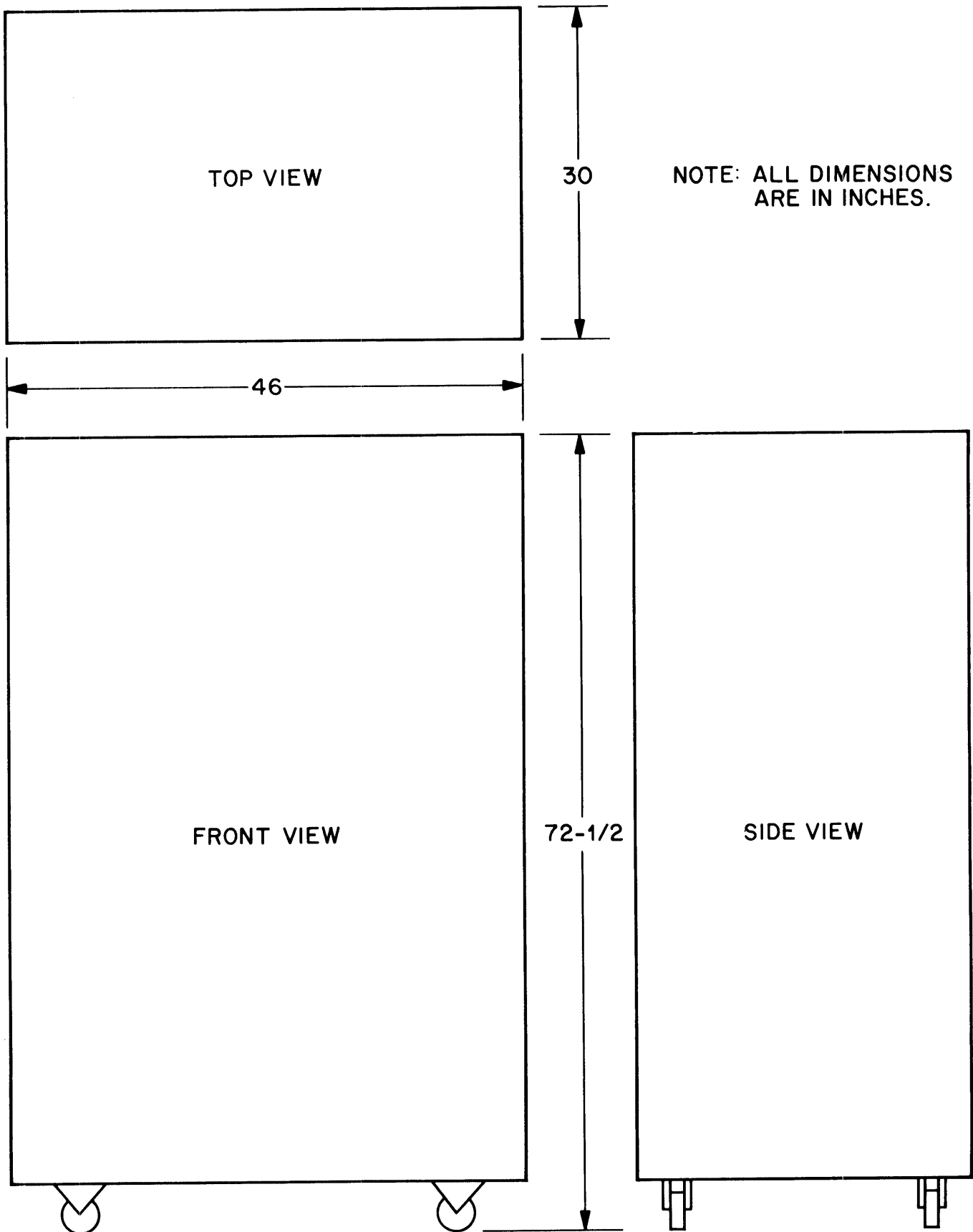
Figure 2-38. HP 2992Z Two-Bay Cabinet Outline Drawing
