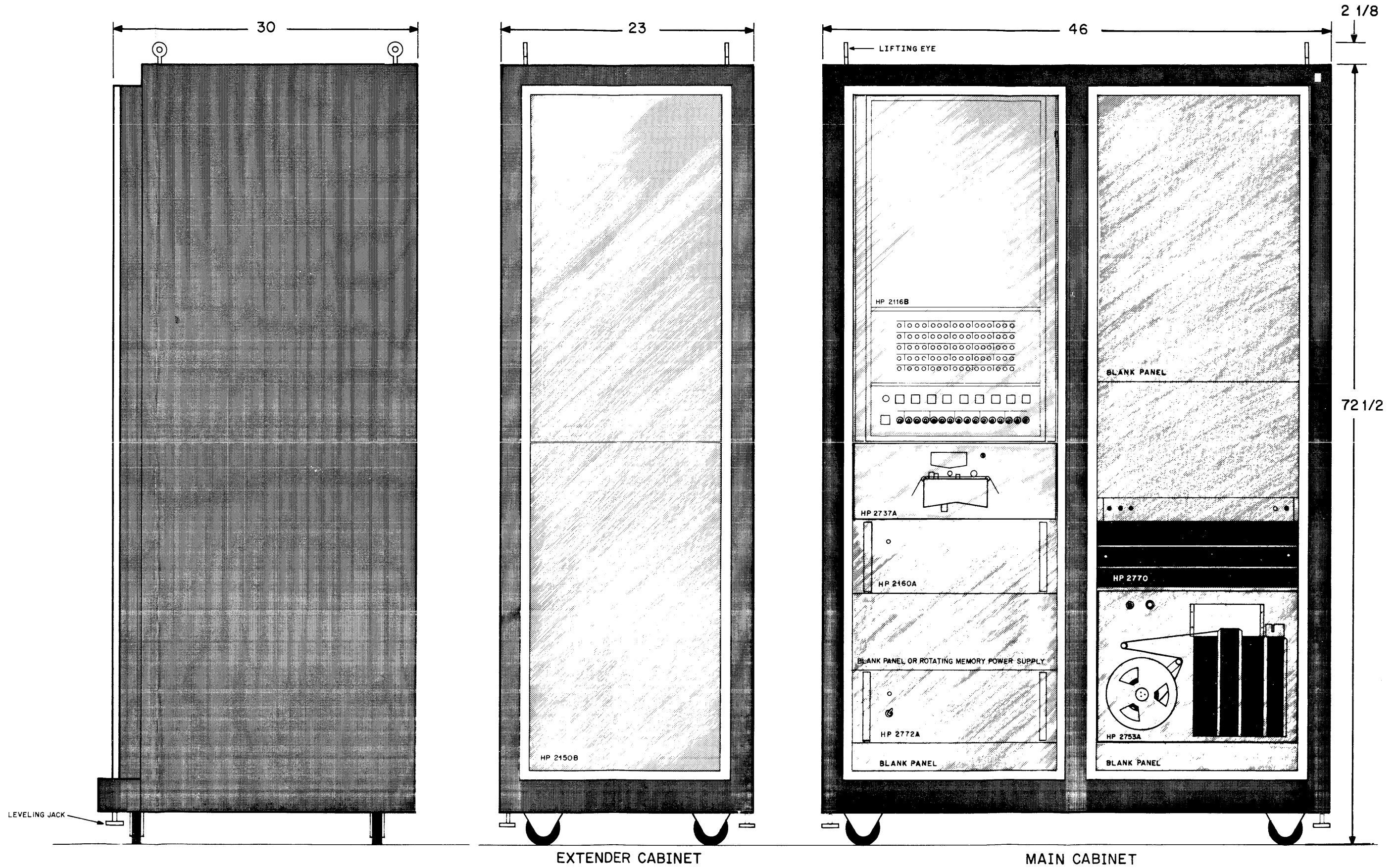
Figure 1-1. Hewlett-Packard 2000A Time-Shared BASIC System
