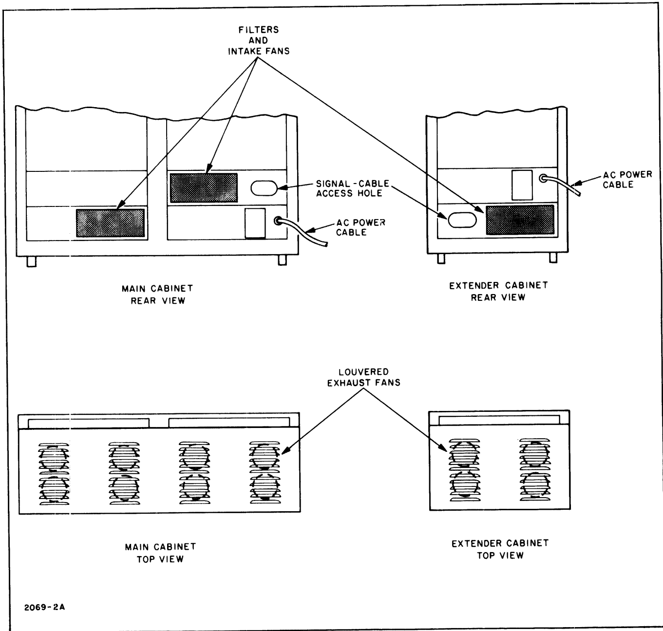
Figure 1-4. System Cabling and Ventilation
