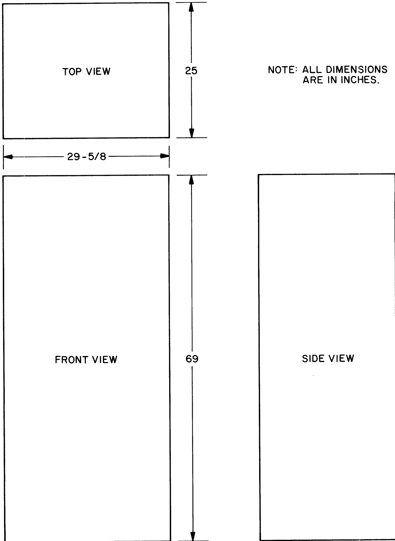
Figure 2-18. HP 3030G Digital Tape Unit Outline Drawing
