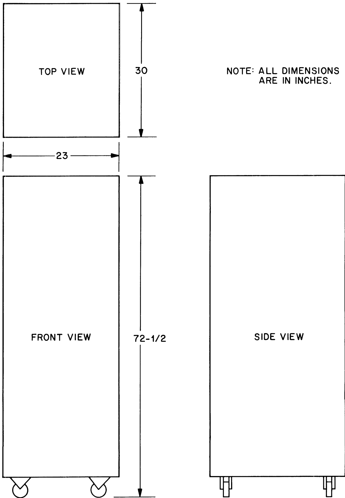
Figure 2-40. HP 2866A Extender Cabinet Outline Drawing
