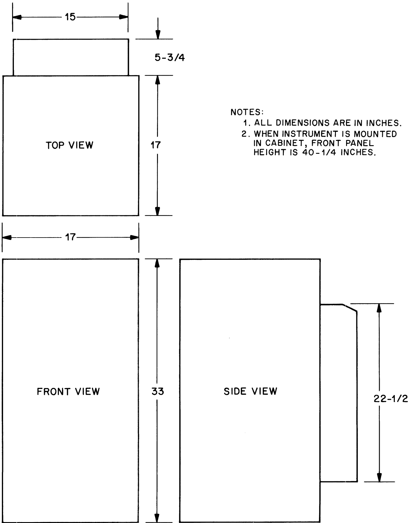
Figure 2-30. HP 2775A Drum Memory Outline Drawing
