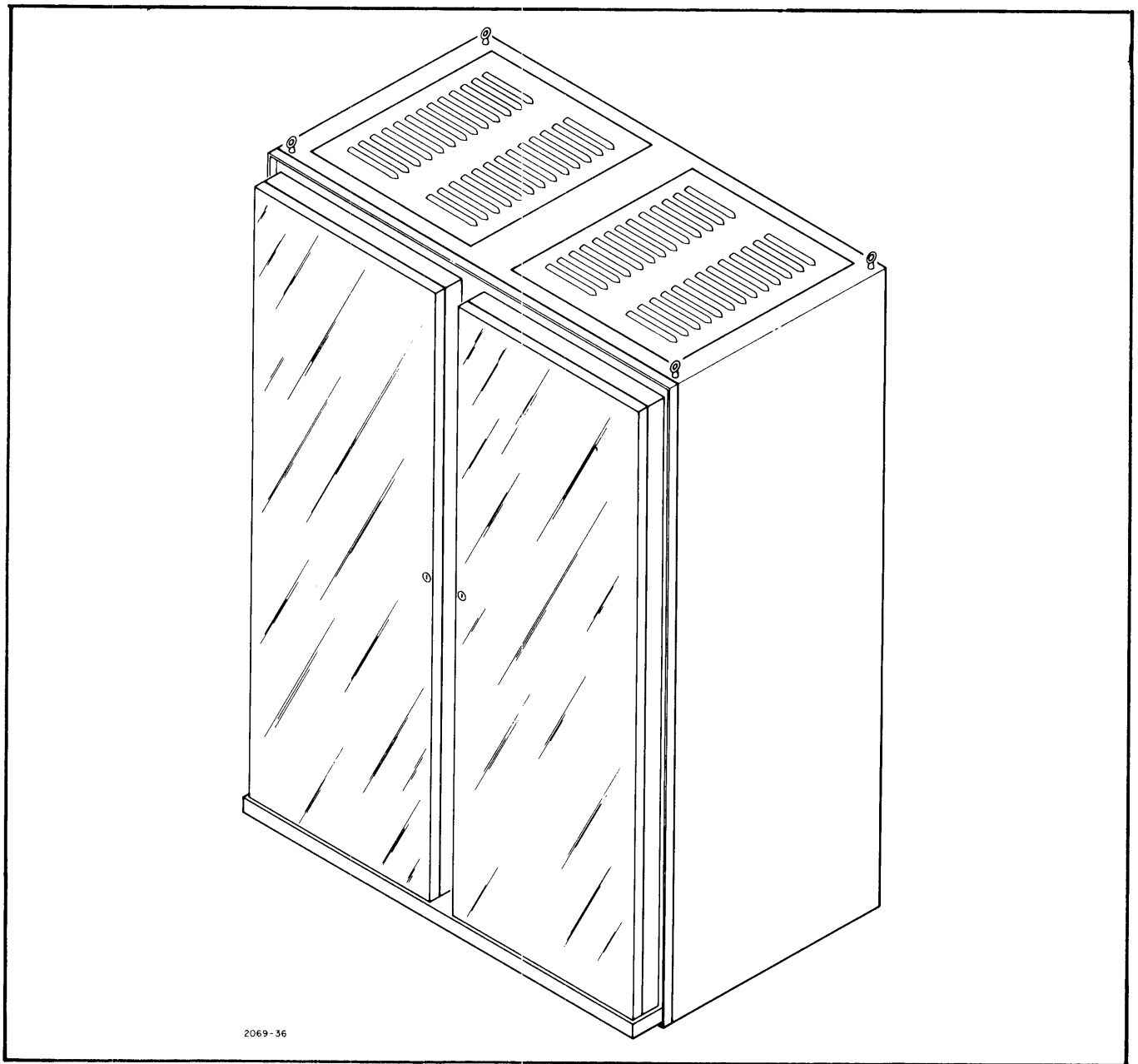
Figure 2-37. HP 2992Z Two-Bay Cabinet
