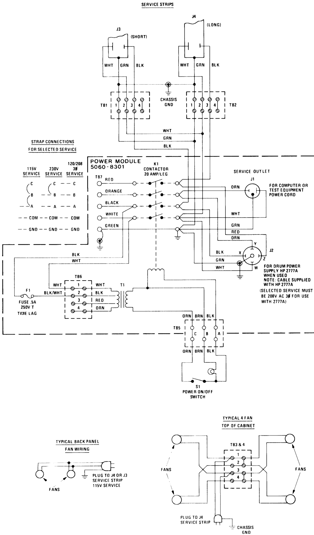
Figure 3-1. HP 2992Z Two-Bay Cabinet Wiring Diagram
